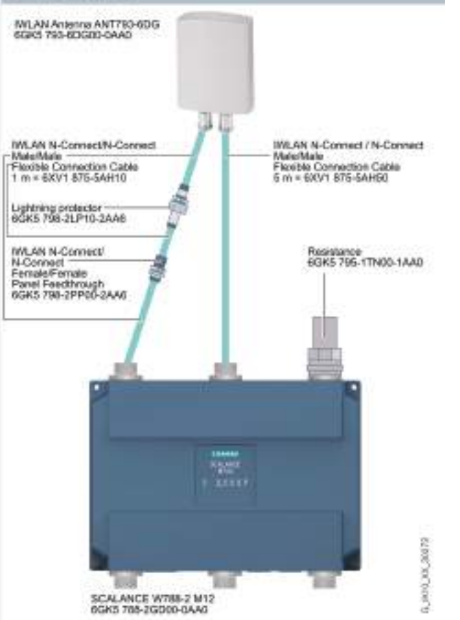
Dual Band antenna ANT793-6DG connected to SCALANCE W788-2 M12 with N-Connect ports
