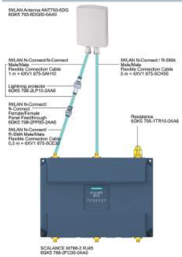
Dual Band antenna ANT793-6DG connected to SCALANCE W788-2 RJ45 with R-SMA ports
